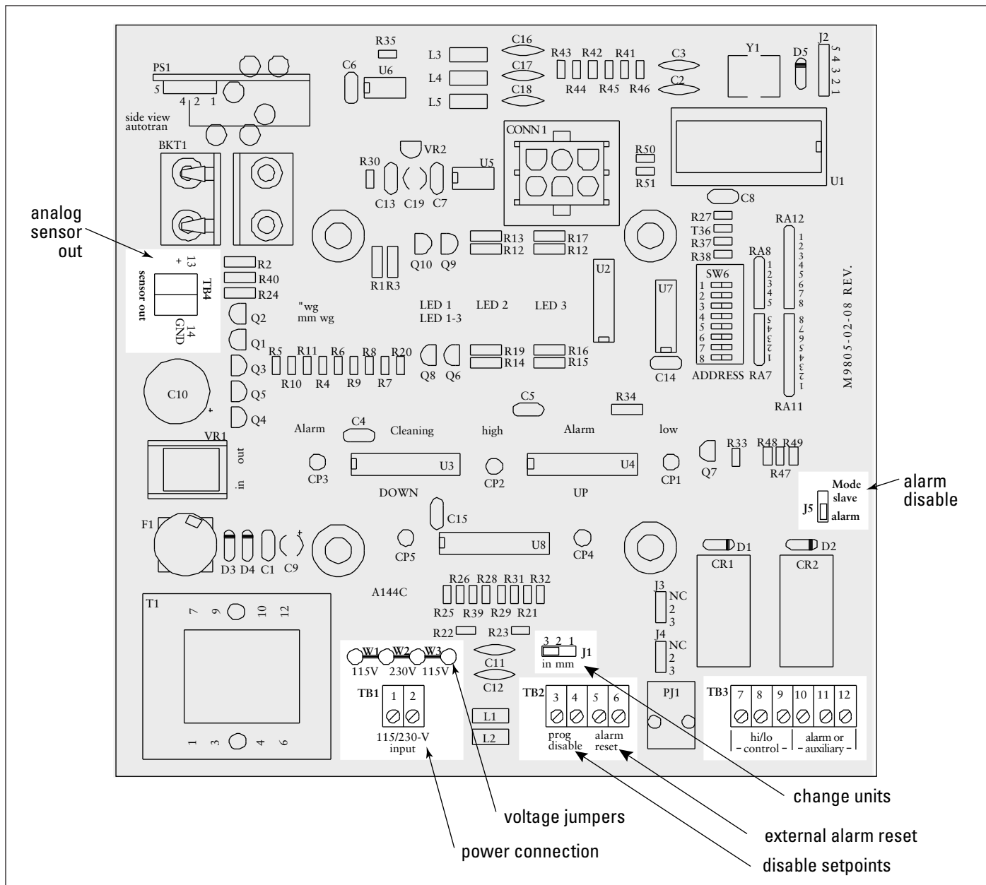
Printed Circuit Board (Optional Settings Location)
