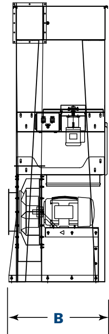
Model 460-IRD-20 Side View
