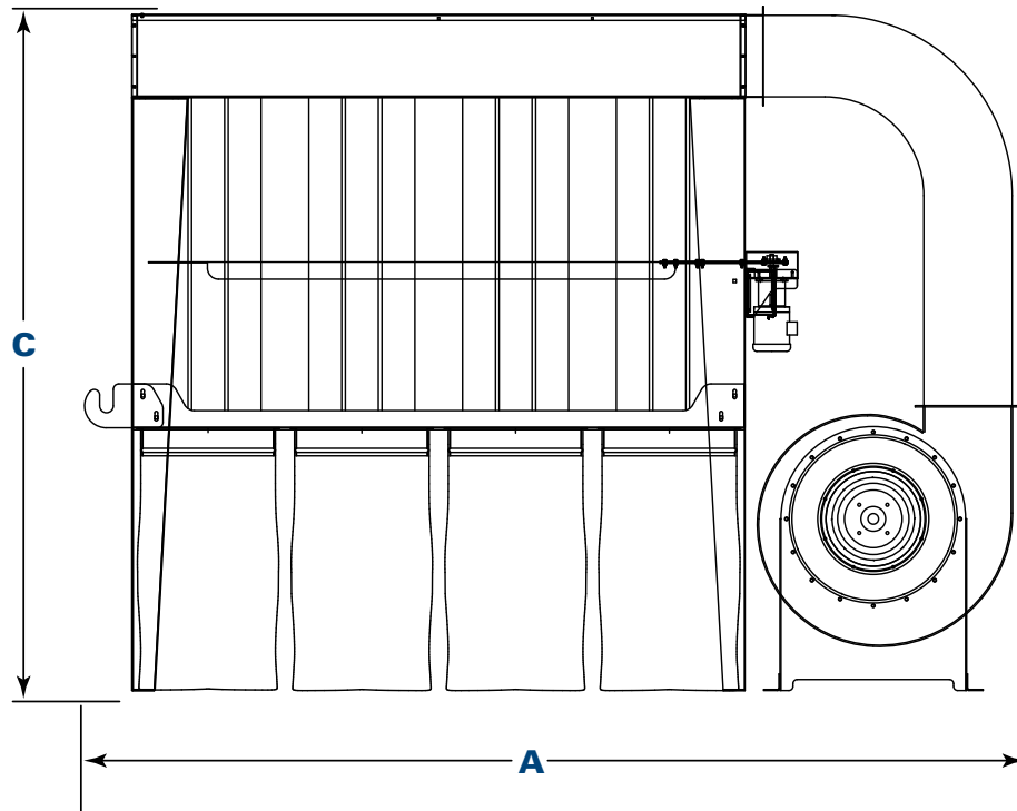
Model 460-IRD-20 (shown w/optional shaker motor) Front View
